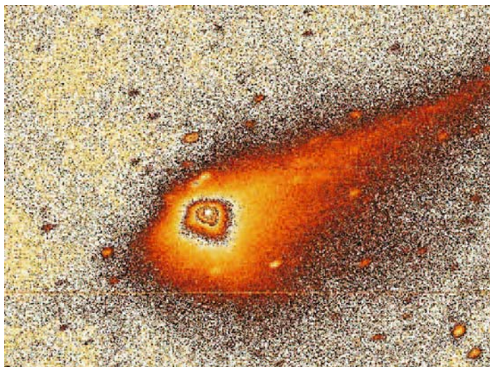
Figure 8. Comet 67P/Churyumov-Gerasimenko at 2.49 AU from the Sun, imaged on March 9, 2004 through broadband R filter with the EFOSC2 instrument at the 3.6 m telescope of the European Southern Observatory in La Silla/Chile. Non-circular isophotes in the coma indicate asymmetric material emission from the nucleus. The tail and neck-line structure extends beyond the edge of the field of view at PA \approx 295^\circ . North is up and East to the left. The field of view is 70,000 \times 50,000 \text{ km}^2 at the distance of the comet. Figure by courtesy of Hermann Boehnhardt and ESO.
