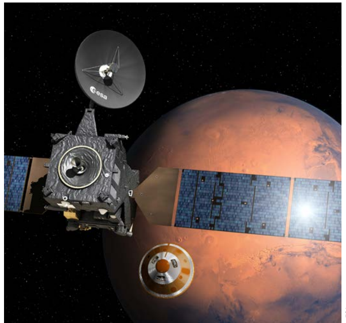
Establishing if life ever existed on Mars is one of the outstanding scientific questions of our time. To address this important goal, the European Space Agency (ESA) has established the ExoMars programme to investigate the Martian environment and to demonstrate new technologies paving the way for a future Mars sample return mission in the 2020’s.
